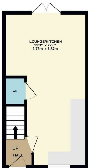
GROUND FLOOR 276 sq.ft. (25.6 sq.m.) approx.
